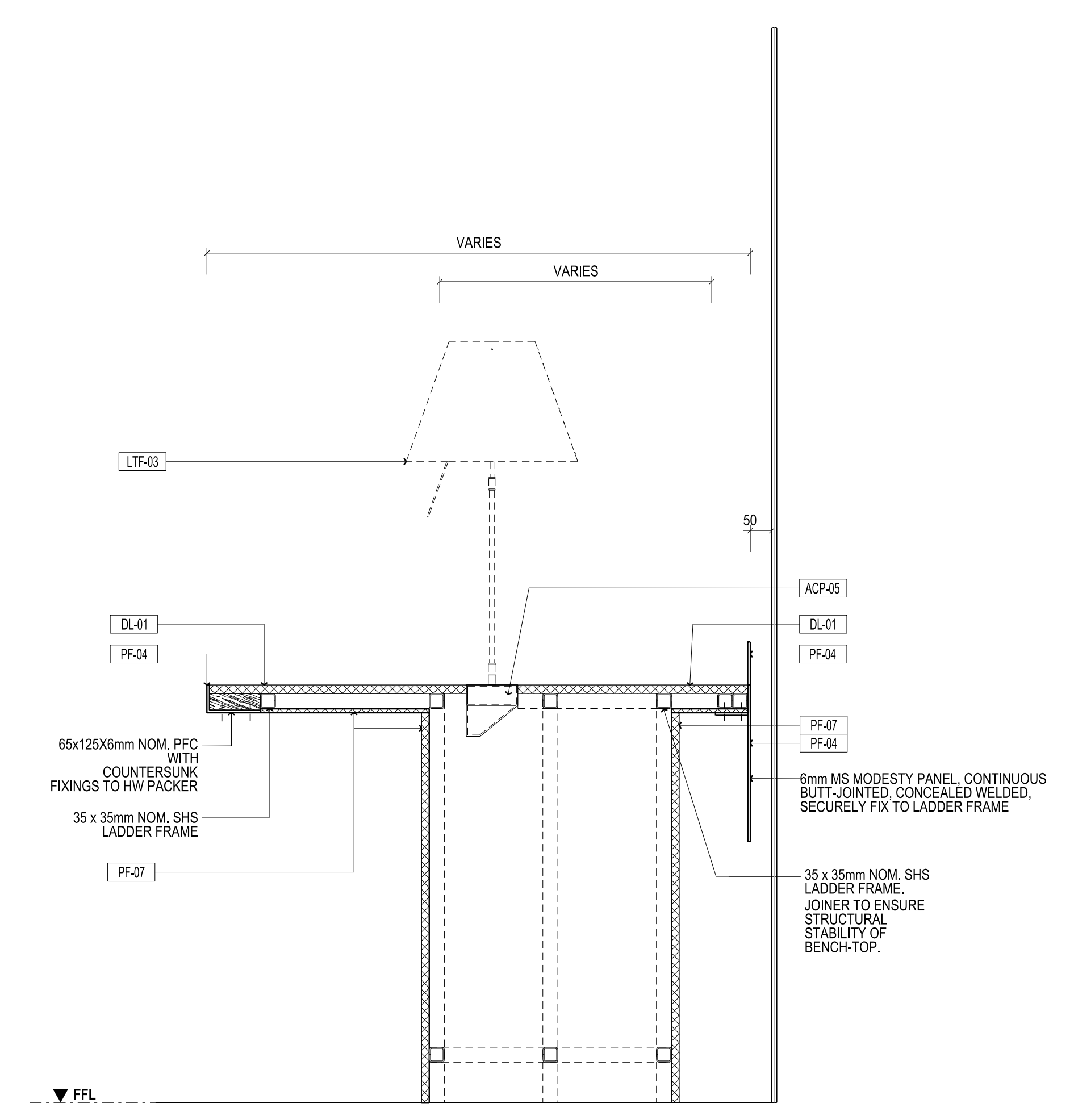
05 DETAIL SECTION - JOG-04 SCALE 1:10
