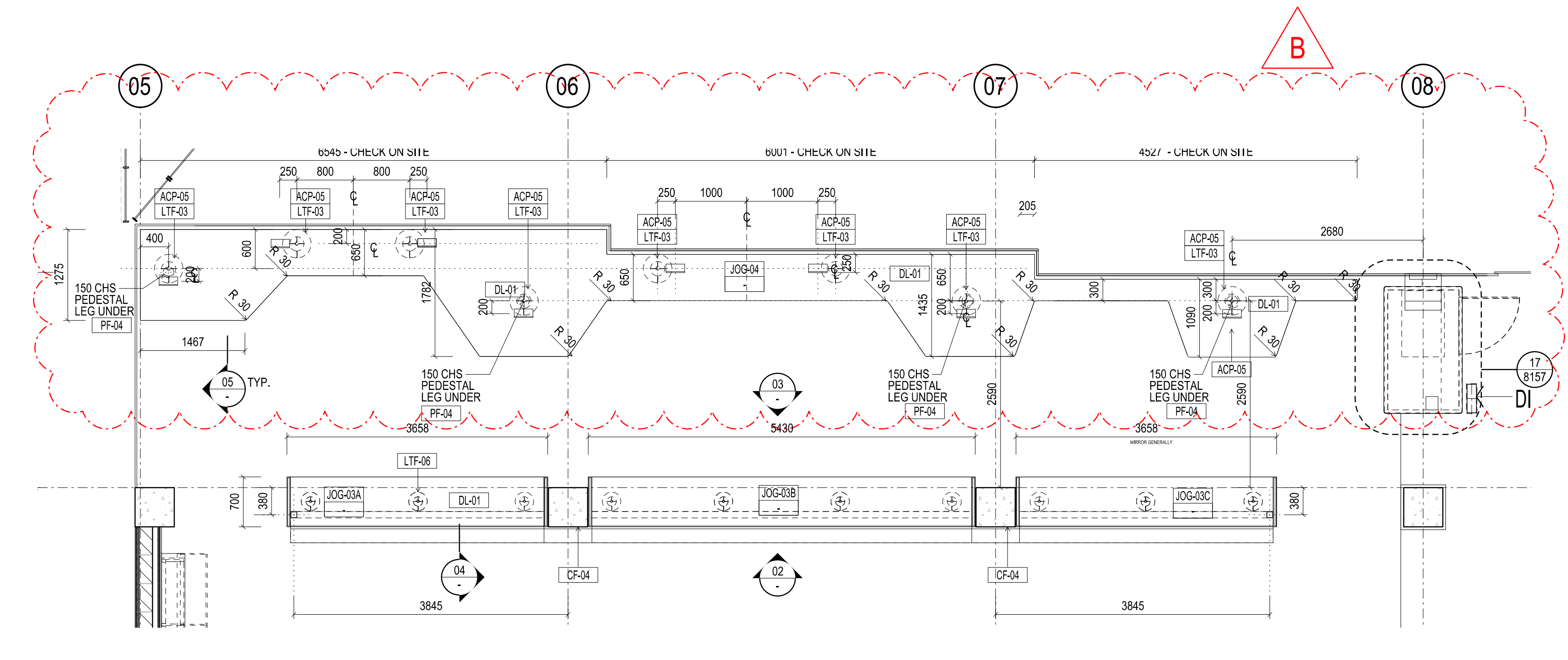
01 PLAN - JOG-03 SCALE 1:50
