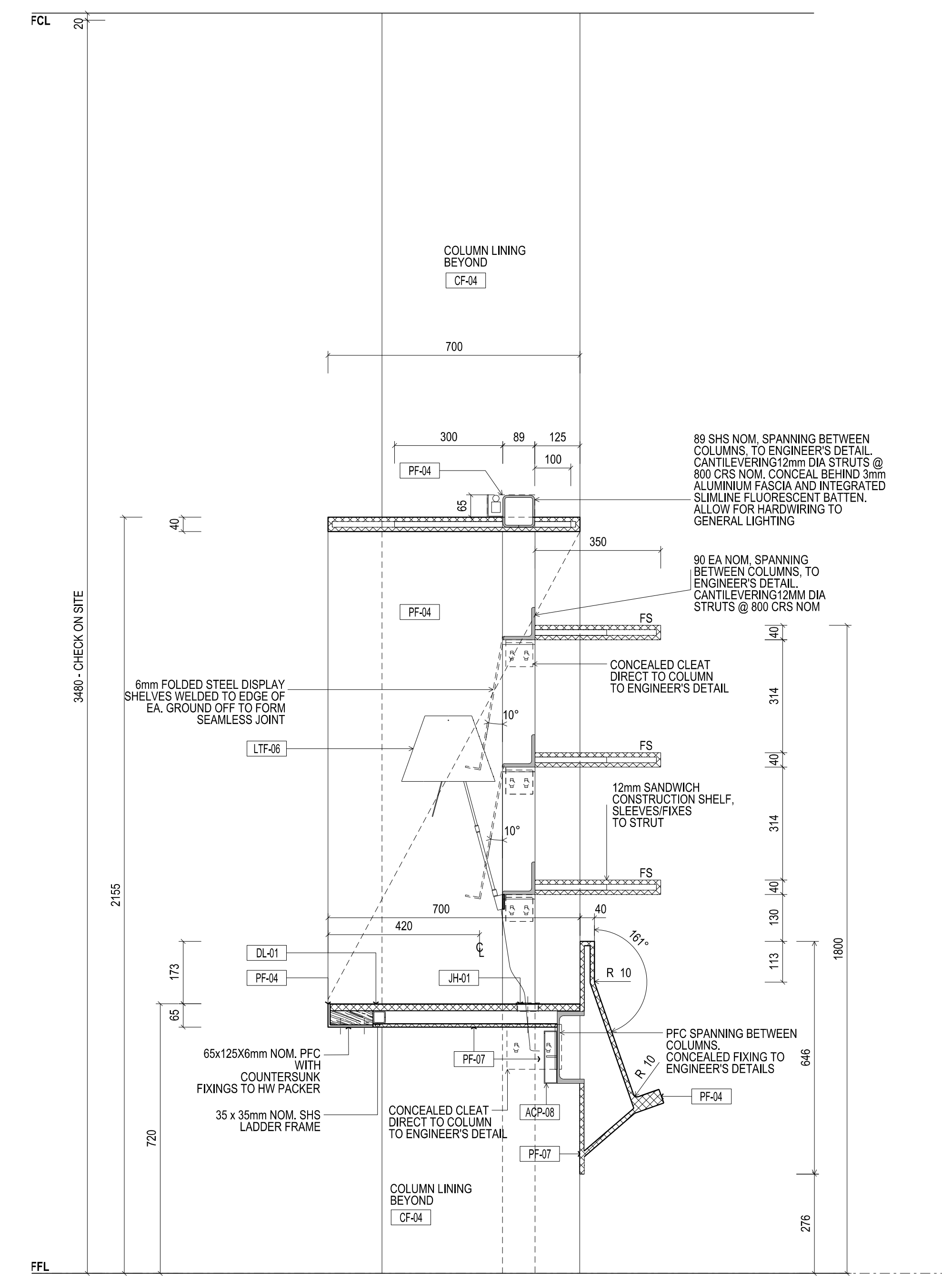
04 DETAIL SECTION - JOG-03 SCALE 1:10
