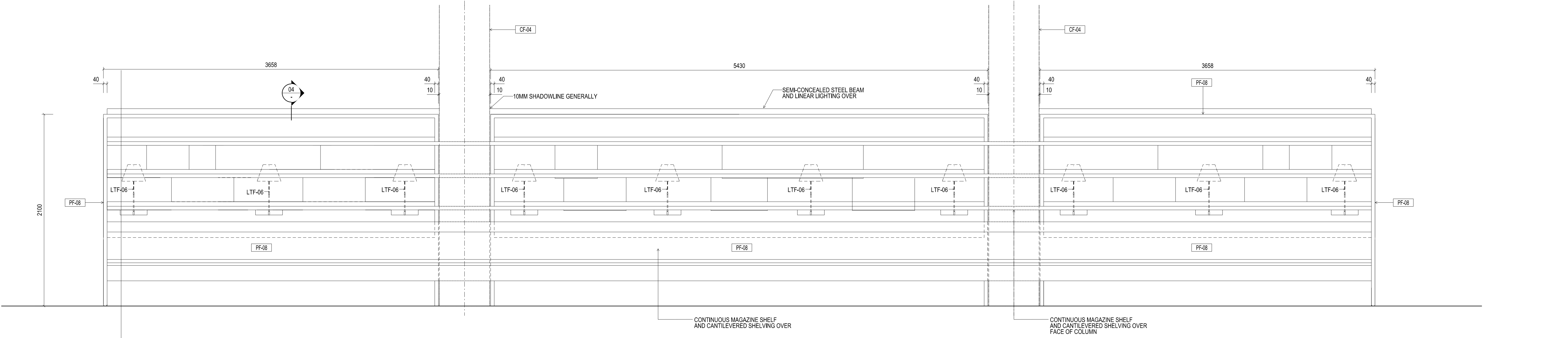
02 ELEVATION - JOG-03 SCALE 1:20
